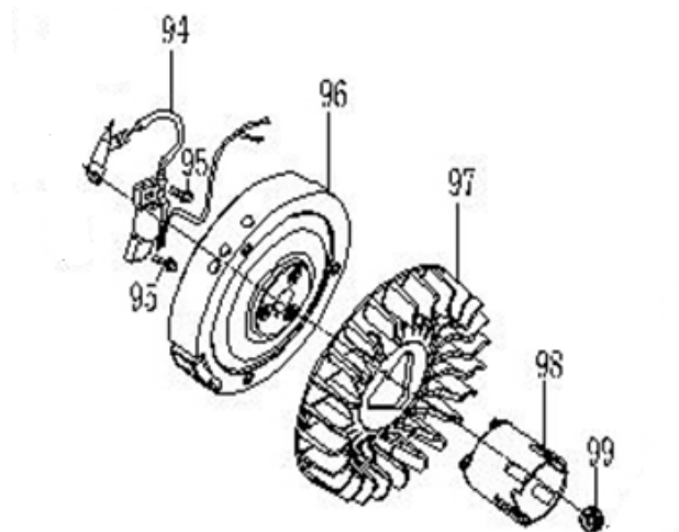
FIG.12 FLYWHEEL ASSY
