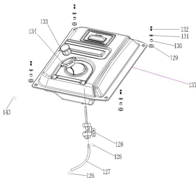
FIG.11 FUEL TANK
