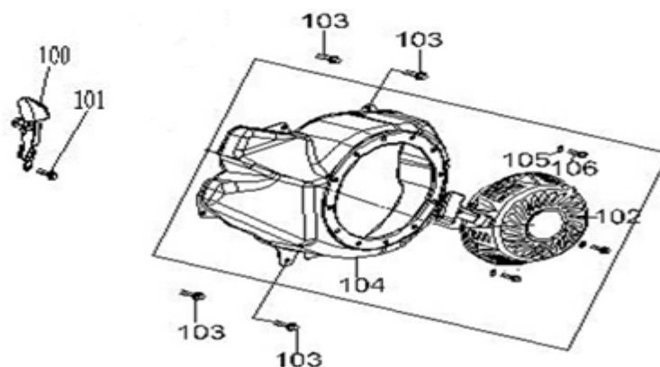
FIG.7 STARTER
