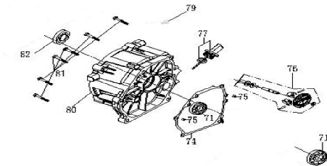
FIG.2 CRANKCASE
