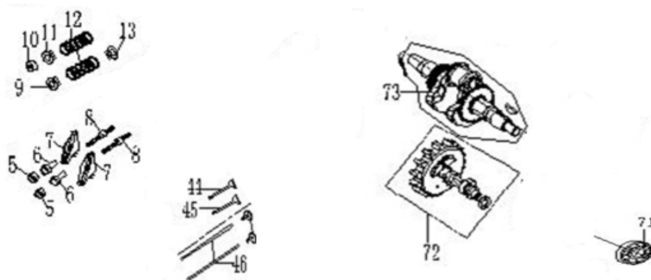
FIG.6 CAMSHAFT ASSY
