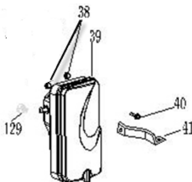
FIG.9 AIR CLEANER
