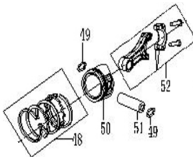
FIG.5 PISTON/CONNECTING ROD
